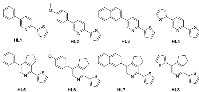
Figure 1. Cyclometallating ligands (protonated) prepared in this study.
