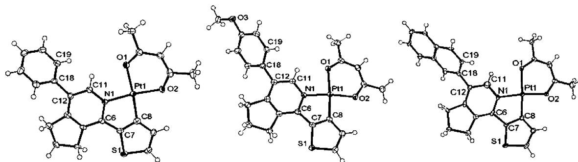
Figure 2. ORTEP drawings of the [Pt(L5)(acac)] (left), [Pt(L6)(acac)] (middle), and [Pt(L7)(acac)] (right) molecules. Selected bond lengths [Å], angles [deg], and torsion angles [deg] are listed in Supporting Information, Table S1.
