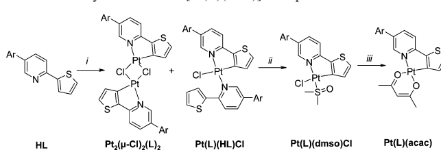
Scheme 2. Synthesis of the [Pt(L)(acac)] Complexes a
